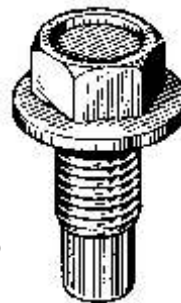
14677 Zinc Thread: M12-1.75 Hex: 15mm Length Under Head: 26mm Washer Head O.D.: 22mm
